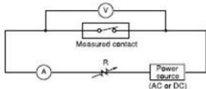
① Ammeter ② Voltmeter ③ Variable resistor
