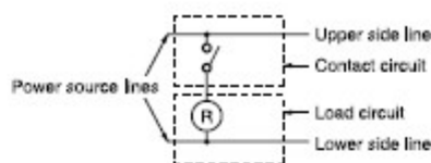
Fig. 5 Example of a vertically written sequence circuit
