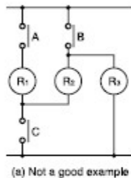
Fig. 5 Example of a vertically written sequence circuit
