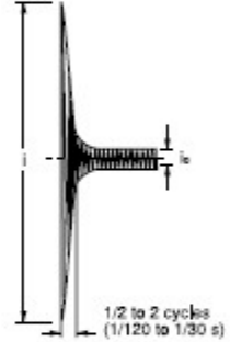
(7) Capacitive Load i/i_0 = 20 to 40 times
