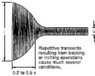
(4) Motor Load i/i_0 = 5 to 10 times
