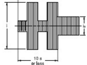
(3) Fluorescent Lamp Load i/i_0 = 5 to 10 times
