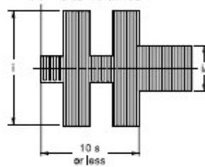
(3) Fluorescent Lamp Load i/i_s = 5 to 10 times
