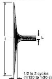
(7) Capacitive Load i/i_s = 20 to 40 times
